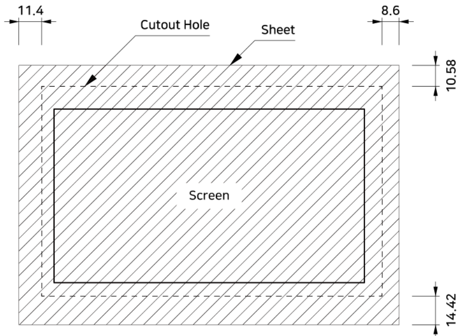
(2) TOPRN0700WD – Flat Mount Front Protective Sheet Drawing
