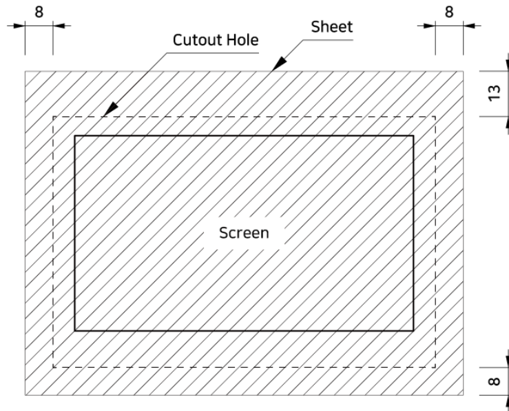
(1) TOPRN0400WD – Flat Mount Front Protective Sheet Drawing
